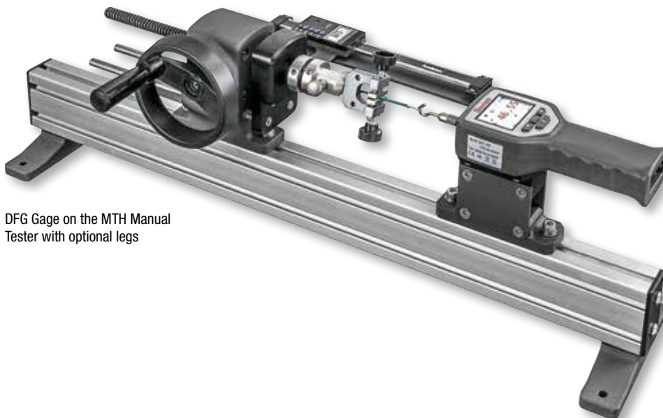
DFG Gage on the MTH Manual Tester
