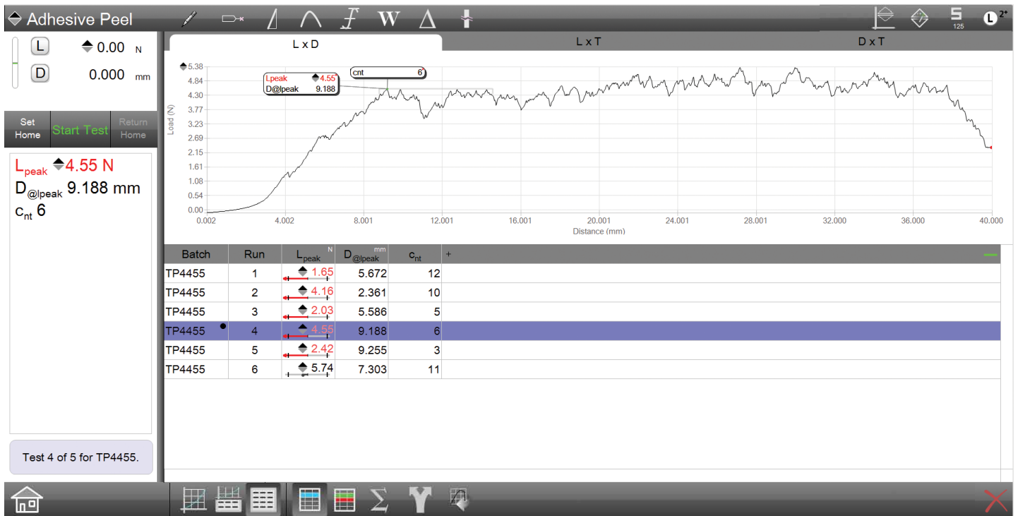
L2 Plus Full Graph view
