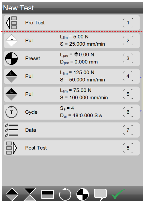
L2 Plus Test Stage Shows multiple step test setup
