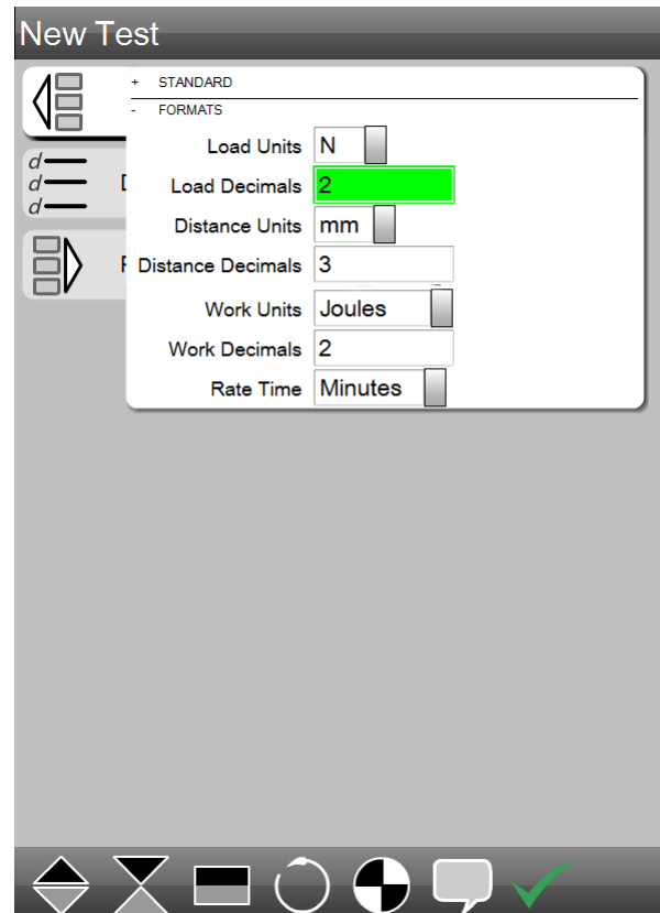
L2 Plus Pre Test Stage FORMATS options and attribute setup
