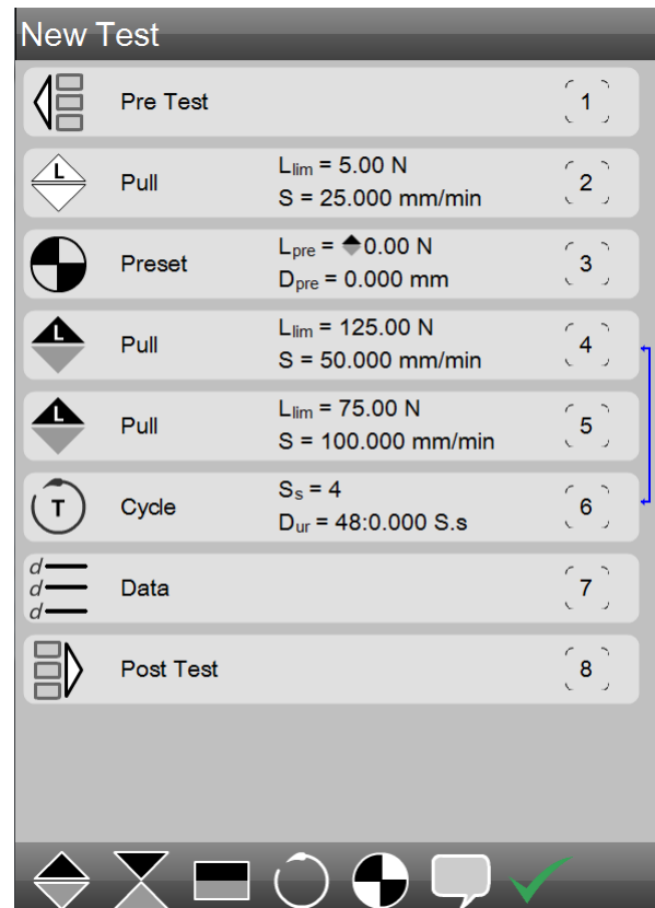
Multi-step L2 Plus Test Setup
